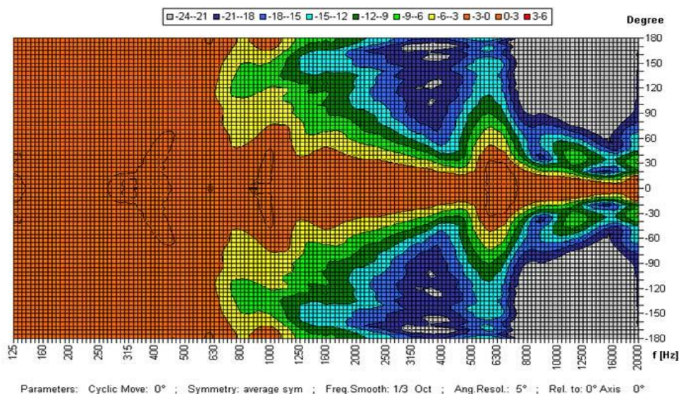
Horizontal Isobars of: ic audio DA-P 20-130T-EN54 Copyright by Four-Audio GmbH & Co KG Licensed to AAC
